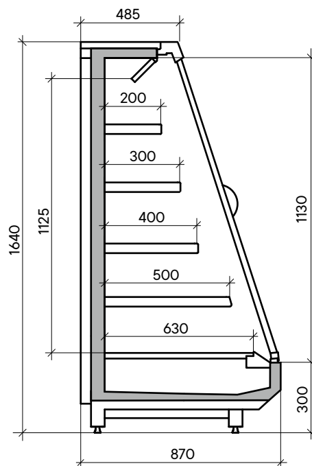
CRETE H-1600 DG Compact
